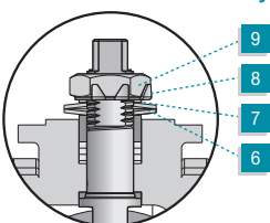
Actuated Valve stem assembly
