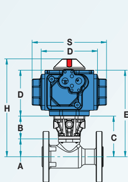
Sizes 1/2" - 1"
