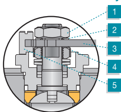
Manual Valve stem assembly
