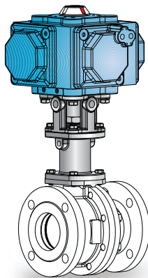
Fugitive Emission with actuator
