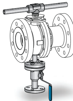
Double Block & Bleed
