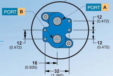
SIDE VIEW C60 - C75
