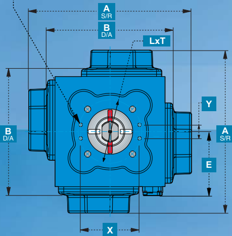
TOP VIEW C60 - C75
