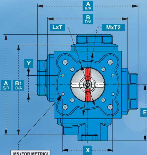
TOP VIEW C15 - C45
