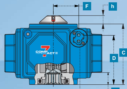
SIDE VIEW C60 - C75
