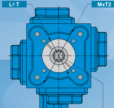
BOTTOM VIEW C15 - C75
